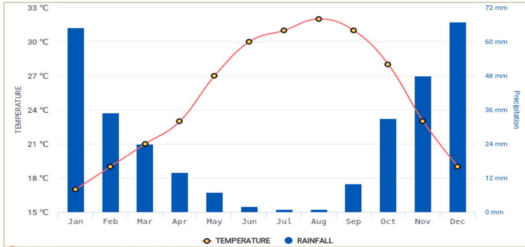
Figure 3: Monthly rainfall rate of study area
