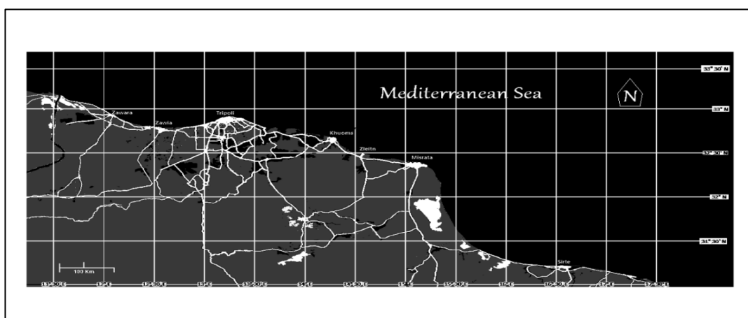
Figure (1): Study location map
