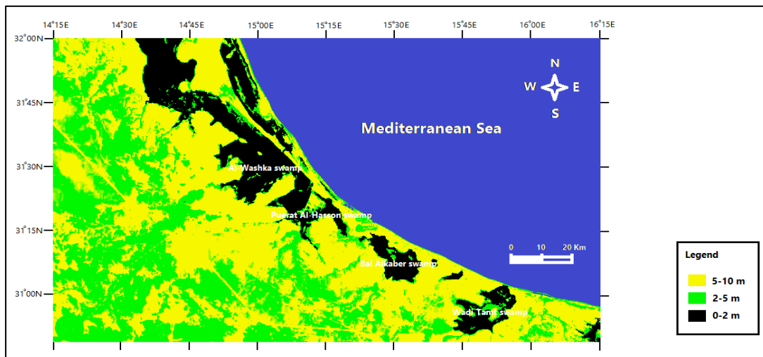
Figure 4: Sabkhas of Sirte .
