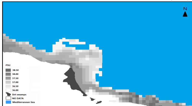
Figure (6,b): Shows the common distribution of August during study period
