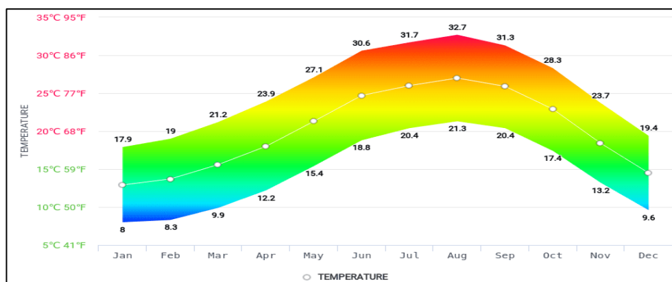
Figure 2: Heat distribution over study location
